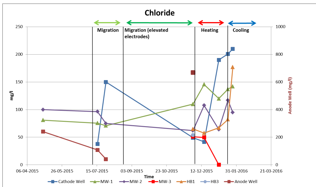
Figure 10.6: Chloride concentrations measured in water samples during the pilot test.
