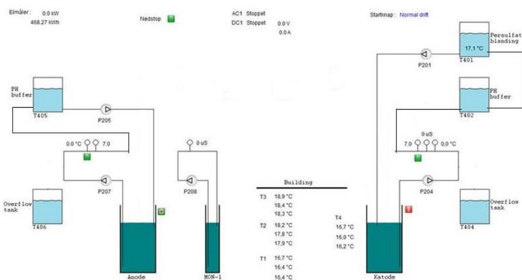
Figure 8.5: PI diagram with adjustments conducted during start-up and initial operation. For higher resolution see Appendix 3.
