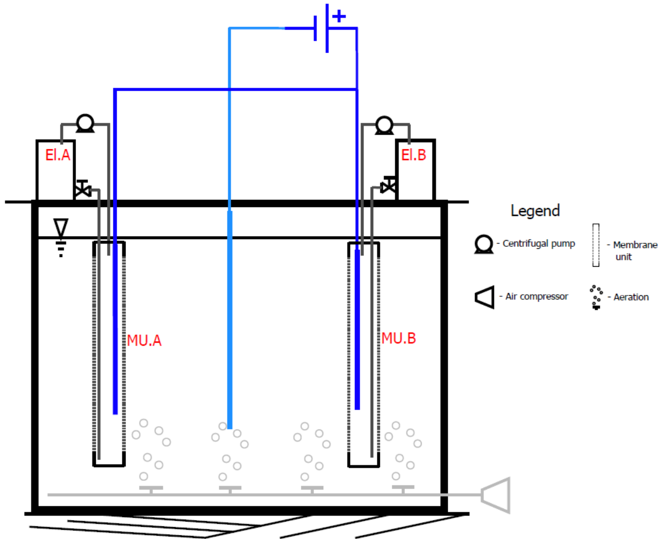
Figure B1 A pilot scale electro-dialytic device to treat soil material suspension, with compressed air applied in a bottom for mixing, membrane units submerged in slurry (MU.A and MU.B) and mixed with remaining electrolyte solutions (El.A and El.B) placed on the top of the tank
